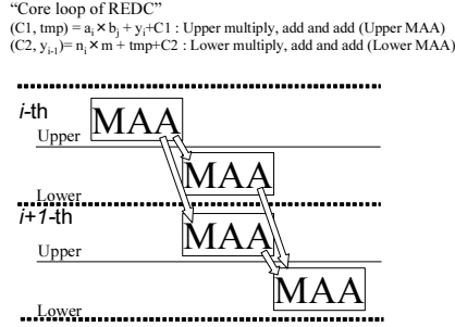
Fig. 2. Pipeline scheduling of “Core loop of REDC” in the Itoh’s algorithm (not optimized to Itanium 2)
