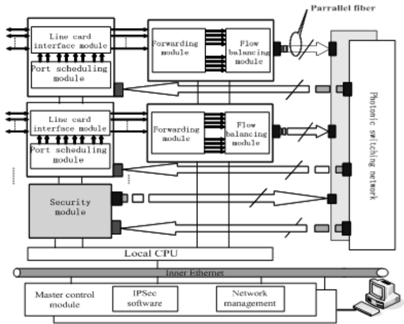
Fig. 2. System Architecture of SR1880S
