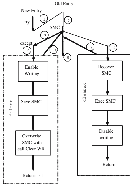
Fig. 8. Program control flow when an SMC occurs
