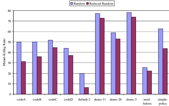
Fig. 3. Mutant-killing ratios for all operators by subjects
