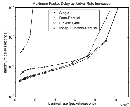
(b) Maximum delay.
