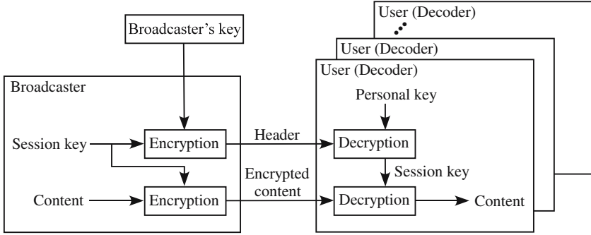
Fig. 1. Content-distribution system
