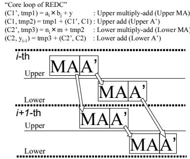
Fig. 3. Pipeline scheduling of “Core loop of REDC” in the Itoh’s algorithm (optimized to Itanium 2)
