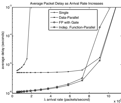
(a) Average delay.
