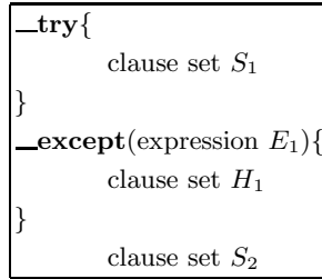
Fig. 2. try-except syntax
