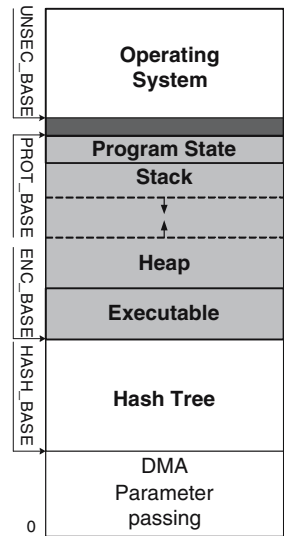
Fig. 1. Memory Layout
