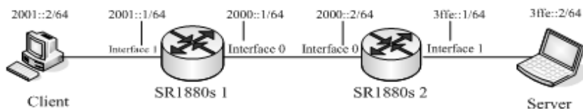
Fig. 9. Architecture of Testing Security Module with Two Routers
